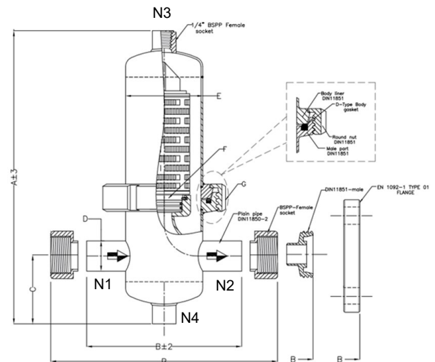
N1: Inlet, N2: Outlet, N3: Connection top, N4: Drain
